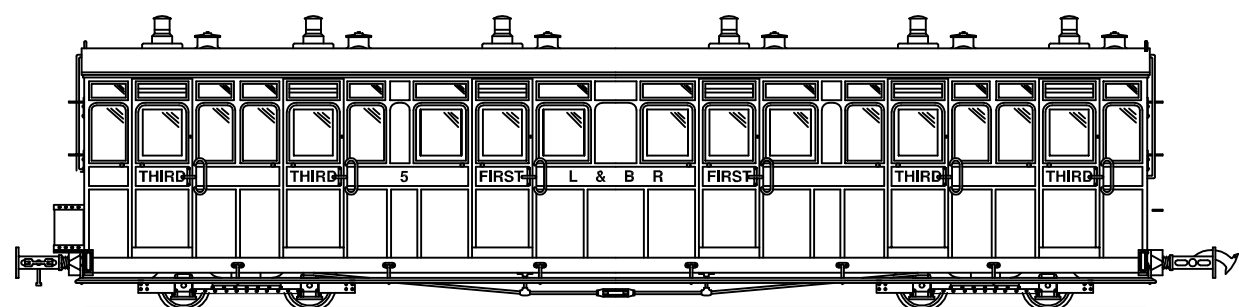
Coaches 5 & 6 Composite
