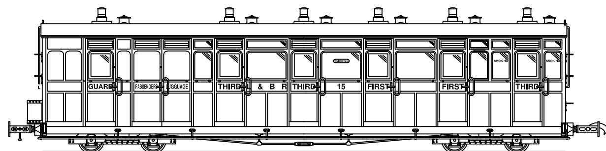
Coach 15 Converted to Brake Composite
