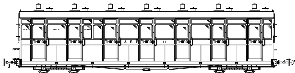
Coaches 11 to 14 Third
