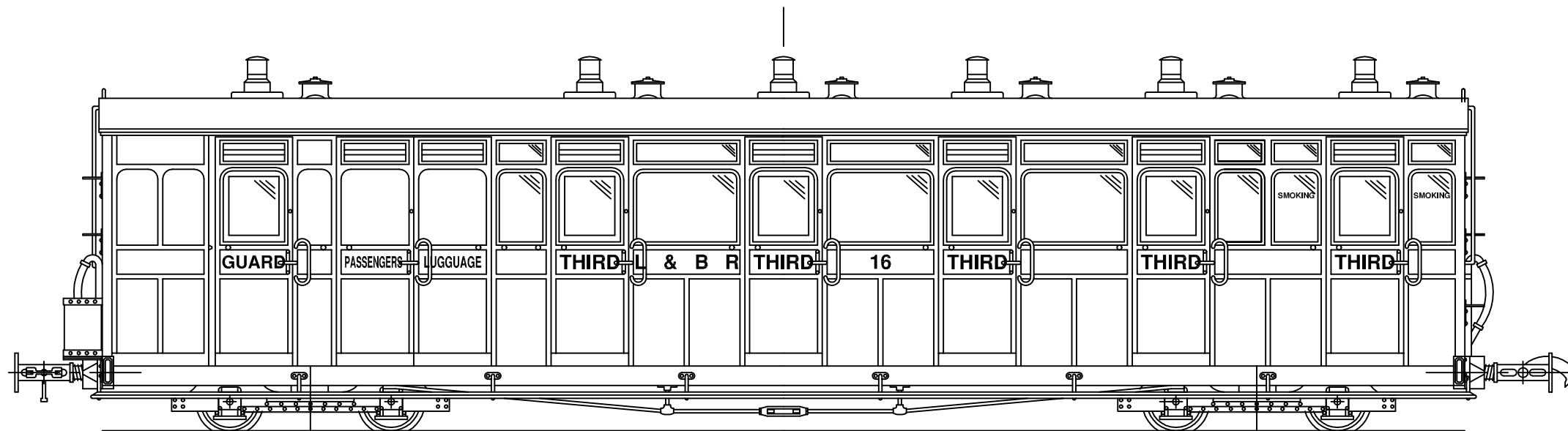
COACH No. 16 - THIRD BRAKE SOUTHERN RAILWAY No. 4108
