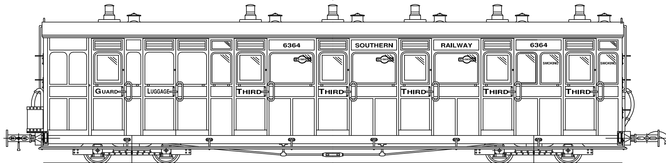
COACH No. 16 - THIRD BRAKE SOUTHERN RAILWAY No. 4108
