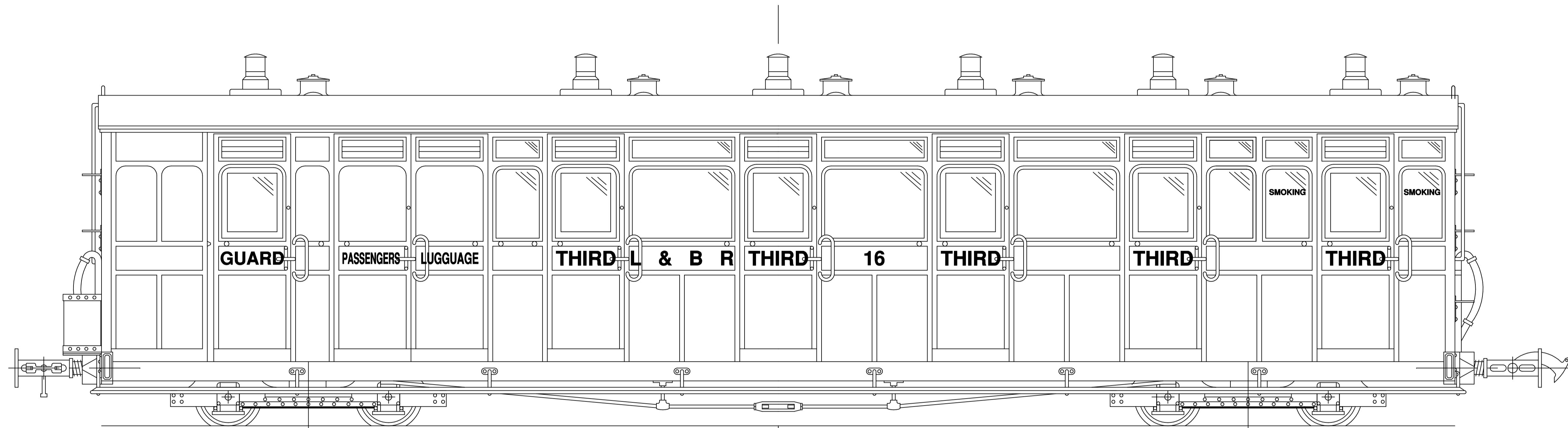
COACH No. 16 - THIRD BRAKE SOUTHERN RAILWAY No. 4108
